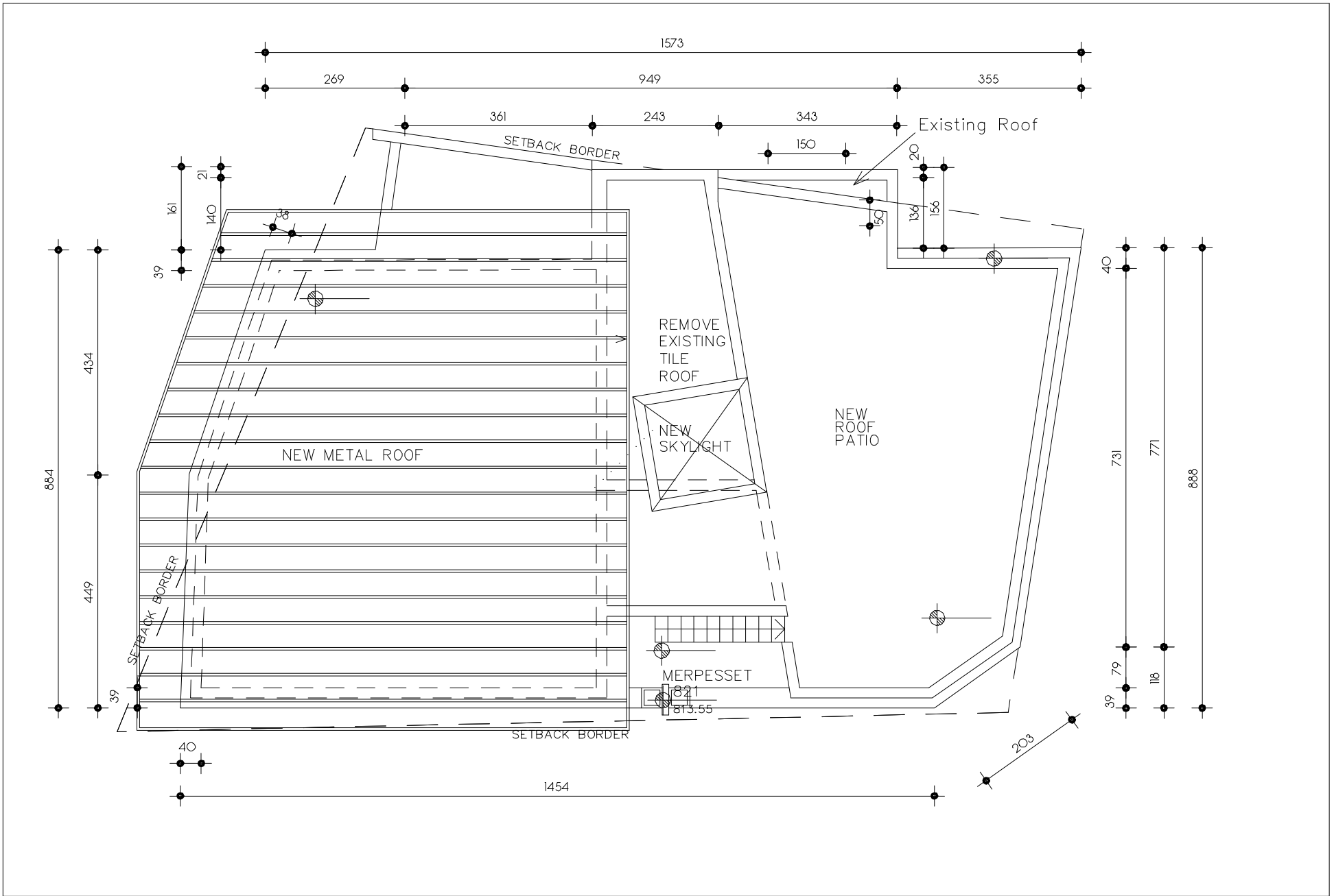
ROOF PLAN
